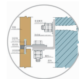
2、不锈钢扣槽式挂件装配示意图 Stainless steel catching groove type hanging fitting
