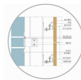
1、背栓式干挂安装示意图 Back bolt type hanging fitting installation schematic layout
