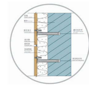
7、无龙骨挂件式装配示意图 Sketch map of keel-less hanging pieces fitting
