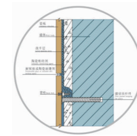
6 无龙骨挂贴式装配示意图 Sketch map of keel-less hanging and sticking fitting
