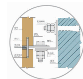
3、不锈钢插销式挂件装配示意图 Stainless steel bolt type hanging fitting
